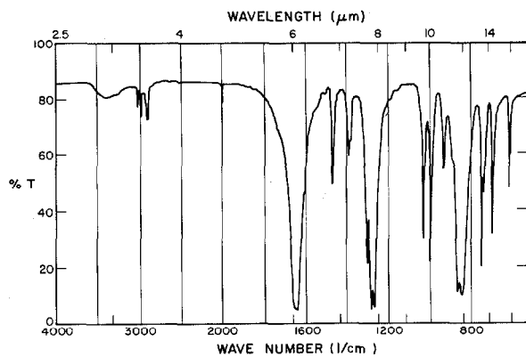
Fig. 1. Infrared spectrum.
